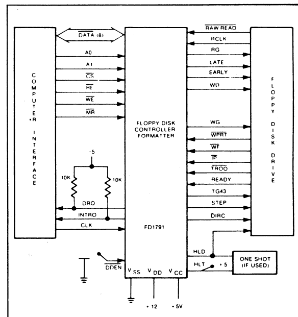
1791 SYSTEM BLOCK DIAGRAM
