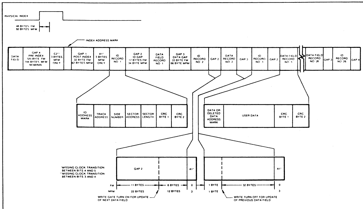
IBM TRACK FORMAT
