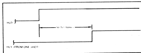
HEAD LOAD TIMING
