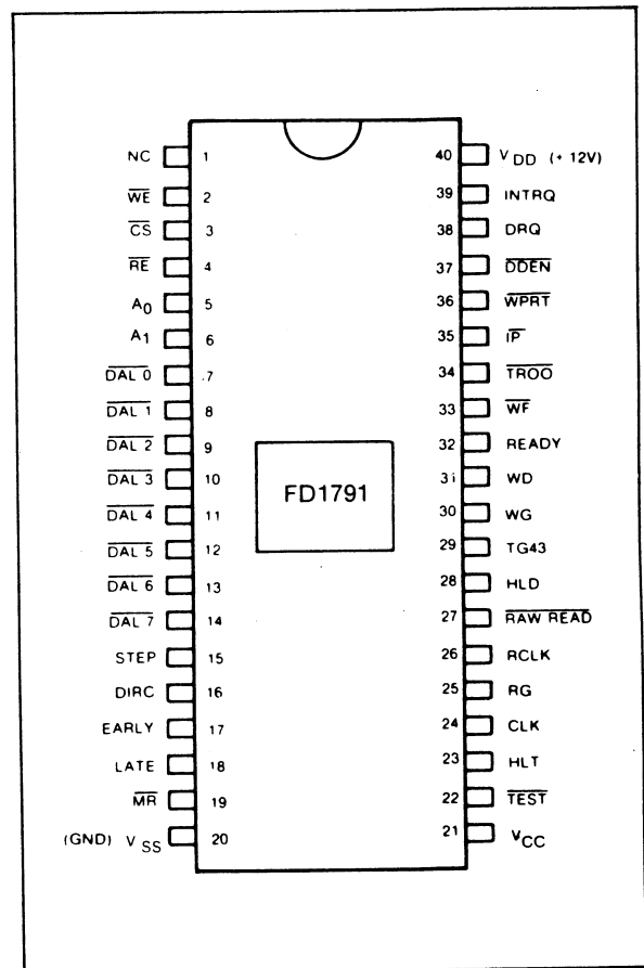
PIN CONNECTIONS
